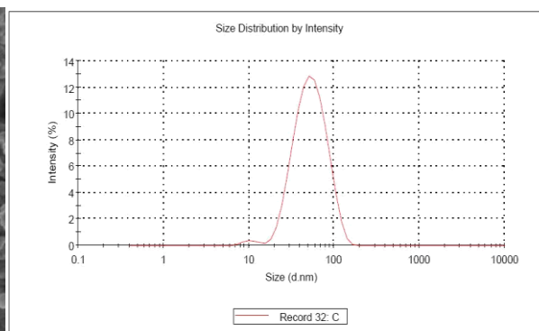
Distribution of NANOSILVER AS 50 - Malvern
