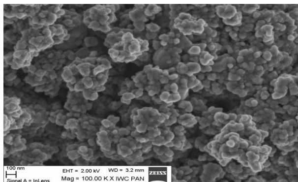
NANOSILVER AS 50 SEM picture
